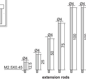
extension rods
